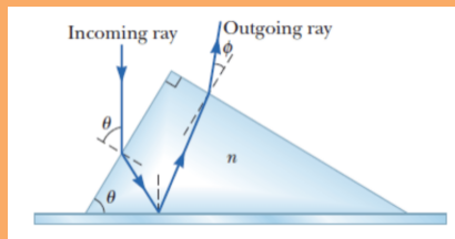
incoming ray
